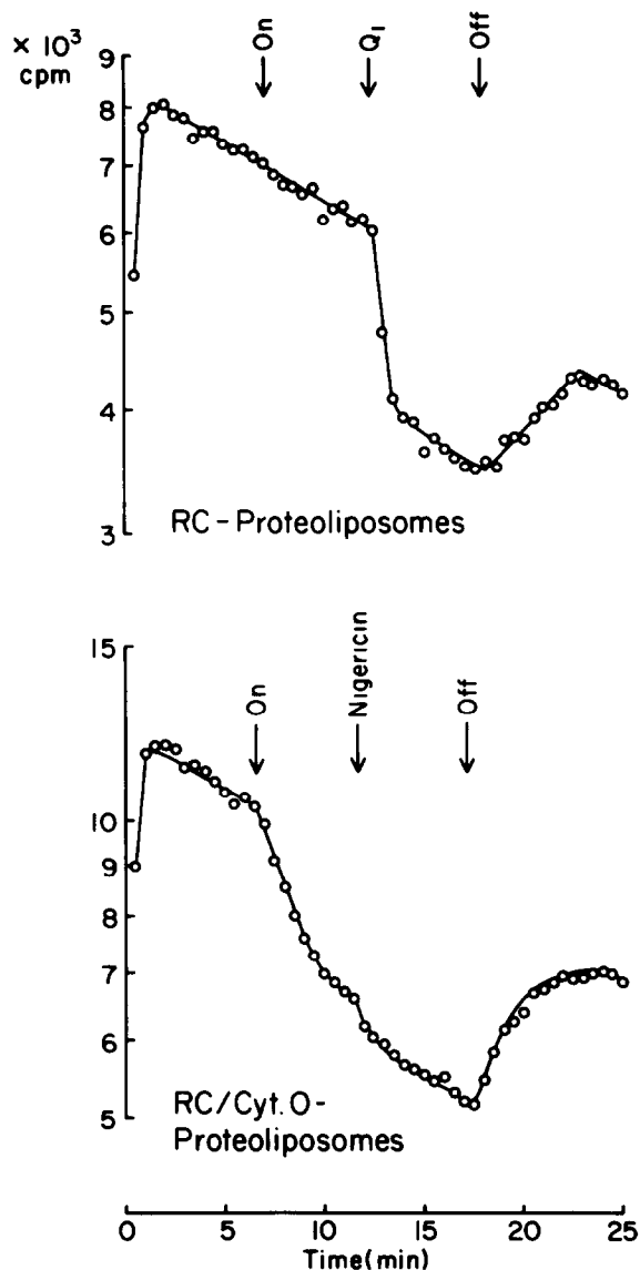
Fig.2. Light-induced transmembrane potential formation in RC or RC/cyt. o hybrid proteoliposomes. [ 3 H]TPP distribution measurements were performed by flow dialysis. The 0.2 ml reaction mixture in 50 mM KPi, pH 7.4, contained either 470 nM RC and 8.3 mM E. coli phospholipids (top trace), or 113 nM cyt. o , 565 nM RC, 8.75 mM E. coli phospholipids and 48.6 \mu M Q 8 (bottom trace). The experiment was begun after the addition of 20 \mu M [ 3 H]TPP (2.5 Ci/mmol) and uptake was initiated by the addition of 10 mM ascorbate/20 \mu M cyt. c . Where indicated, 80 \mu M Q 1 or 0.25 \mu M nigericin was added.
